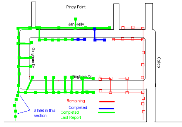
Drawing of the storm lines for Jan Kelly, Calico and Gingham area. Blue is completed this period; Green past weeks and red is still remaining to be done.
